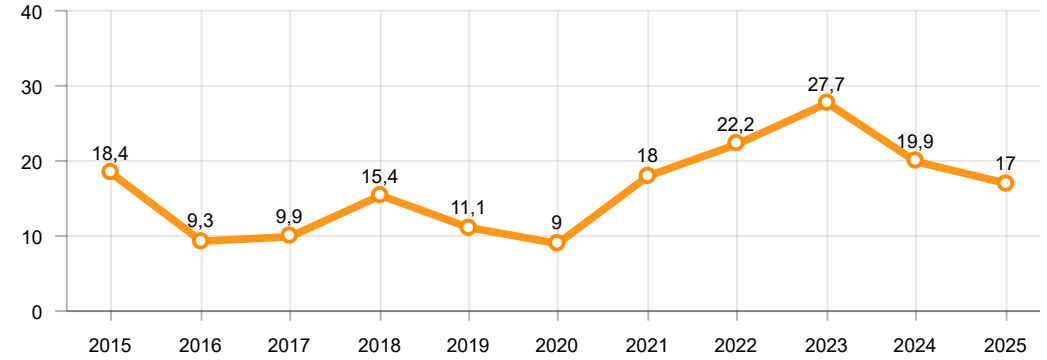
Büyük Kamyon Üretimi (x1000)(OCAK - TEMMUZ) Heavy Truck Production (x1000)(January - July)
